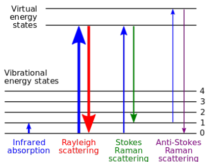
Figure 4: Representation of Rayleigh and Raman Scattering
