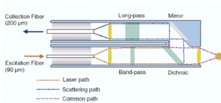
Figure 11: B&W Tek Raman Probe Design (Permission Granted)
