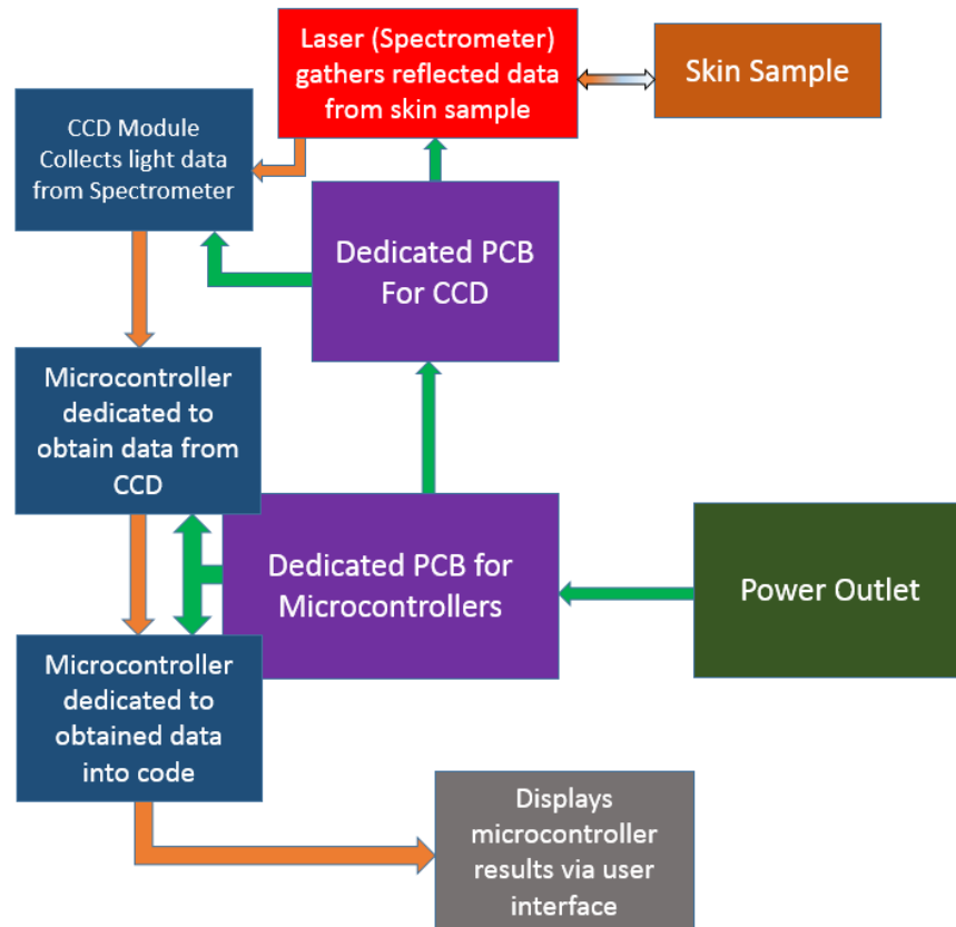
Figure 1: Data and Power Flow Design
