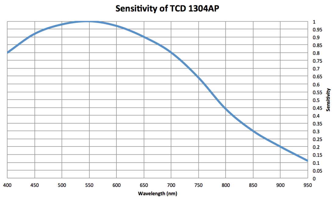
Figure 14: Plot of Sensitivity of TCD 1304AP, information from Data Sheet [21]
