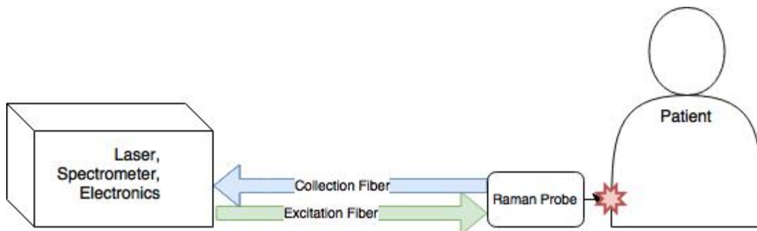
Figure 10: Design Concept for the Raman System
