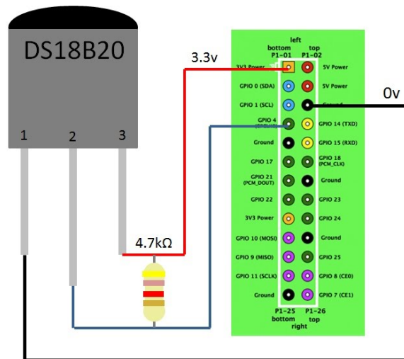
Figure 9: Temperature Sensor
