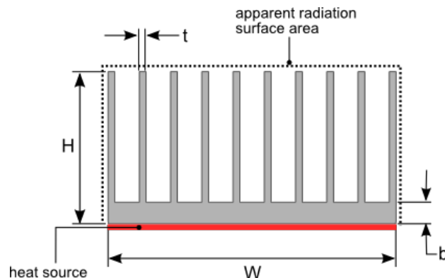
Figure 6: Heat Sink Template
